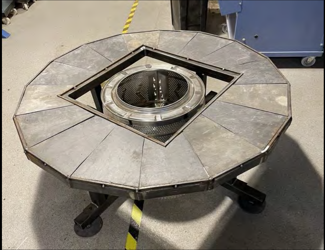
Krish Stanley (2023) Project title – Firepit table
